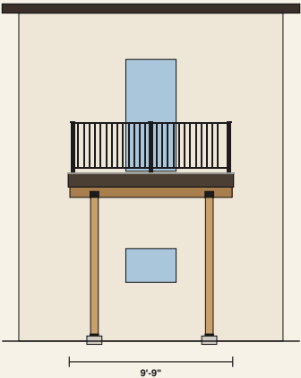
FRONT ELEVATION — from the yard
