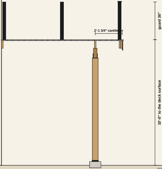
SECTION through zone A at 4'-10 1/2" — looking toward the left end
